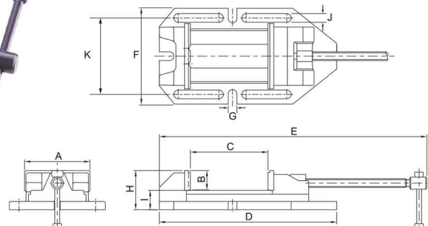
DESIGN FOR THIN & ROUND WORKPIECE
